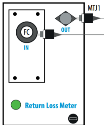
Figure 2- MTJ1 referencing for typical measurements
