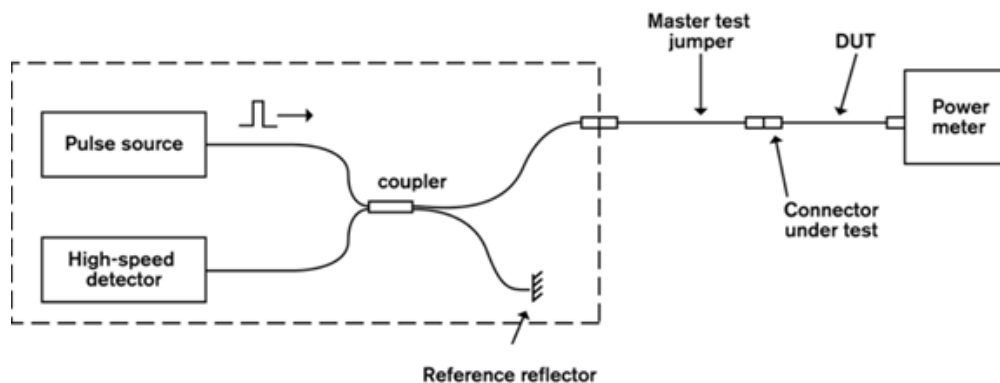
Figure 1- MS12 Single-mode Return Loss Meter general operating principle
