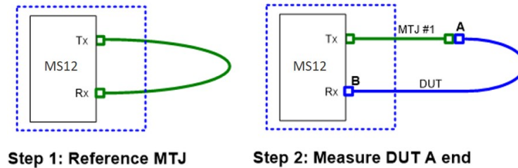
Figure 3- Typical testing sequence with MS12001
